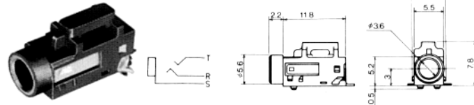
No.MJ-158L (3.5φ) PANEL MOUNT 3-CON. STEREO MINIATURE JACK. (SINGLE CLOSED) Net Weight : 2 gr.
