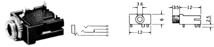
No.MJ-352W-0 (3.5φ) STEREO
