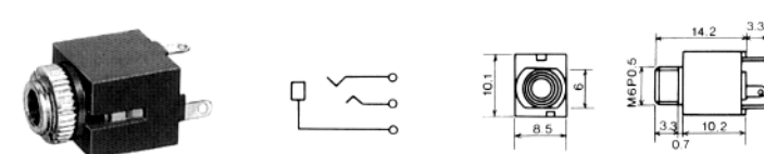
No.MJ-355W (3.5φ) CHASSIS MTG. STEREO JACK
