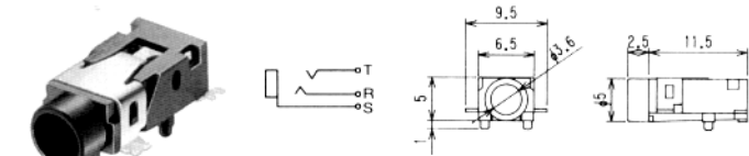
No.M03-292J1 (3.5φ) STEREO
