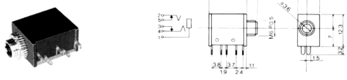
No.MJ-354W-SG (3.5φ) STEREO
