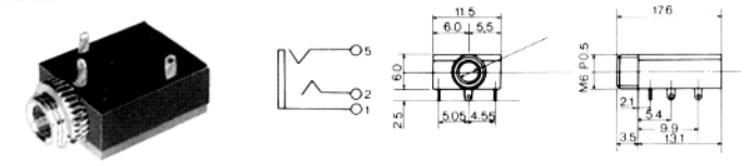
No.MJ-352W-C (3.5φ) STEREO
