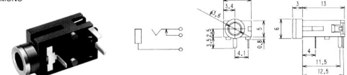
No.MX-328BL (3.5φ) MONO Net Weight : 1.5 gr.
