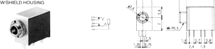
No.MJ-355W (3.5φ) CHASSIS MTG. STEREO JACK
