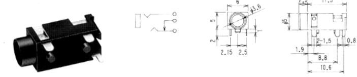
No.MJ-3235 (3.5φ) MONO
