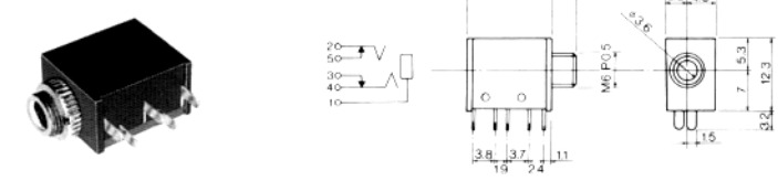
No.MJ-354W-S2 (3.5φ) STEREO JACK FOR P.C. W/SHIELD HOUSING
