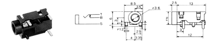
No.MJ-2235 (3.5φ) MONO
